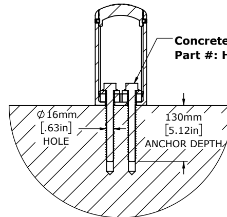
Fixing Detail
